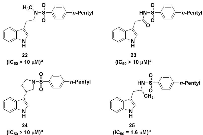
Figure 2. SAR of the linker group. a Enzyme inhibition measured in the presence of LA as substrate.
