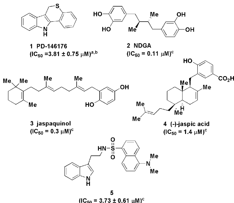
Figure 1. Some known inhibitors of 15-LO and dansyl tryptamine 5 . a Enzyme inhibition measured in the presence of LA as substrate. b Standard deviations are based on multiple test occasions ( n \geq 2 ). c As reported in the literature. 12,13
