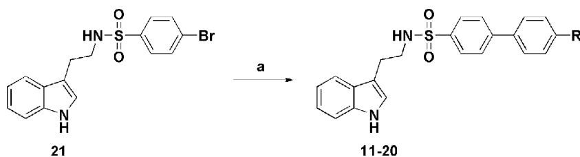
Scheme 1. Reagents and conditions: (a) \text{ArB(OH)}_2 , \text{Na}_2\text{CO}_3 , ethanol/toluene (1:1), \text{Pd(PPh}_3)_4 (65–85%).
