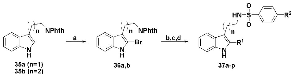
Scheme 2. Reagents and conditions: (a) pyridinium tribromide, THF, \text{CHCl}_3 (73%); (b) \text{R}^1\text{B}(\text{OH})_2 , LiCl, \text{Na}_2\text{CO}_3 , ethanol/toluene (1:1), \text{Pd}(\text{PPh}_3)_4 (5 mol %) (30–75%); (c) \text{NH}_2\text{NH}_2 , MeOH (80–95%); (d) p\text{-(R}^2\text{)PhSO}_2\text{Cl} , \text{Et}_3\text{N} , \text{CH}_2\text{Cl}_2 (95%).
